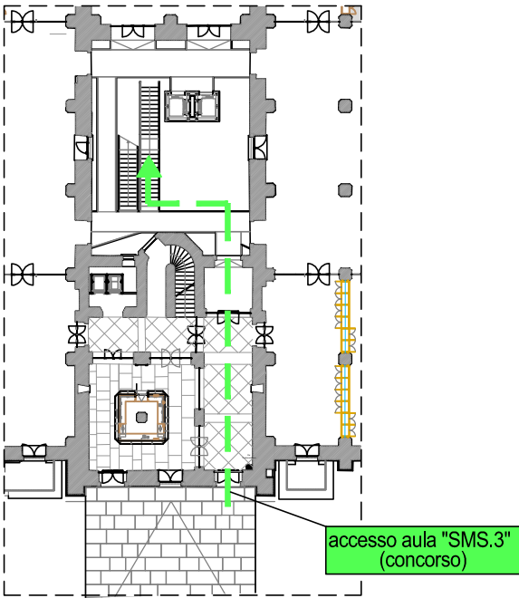
PIANO TERRA
